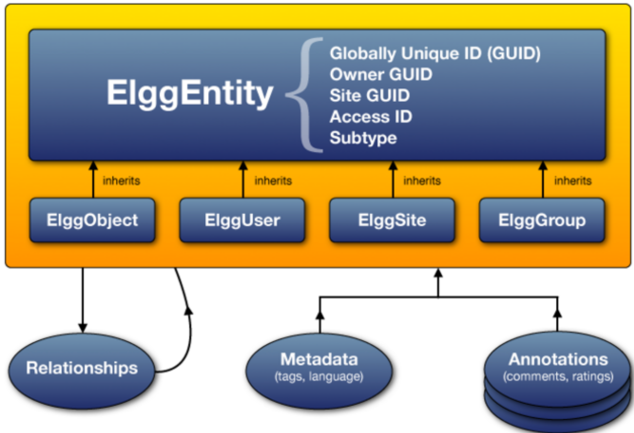
Abb. 9: The Elgg data model diagram
