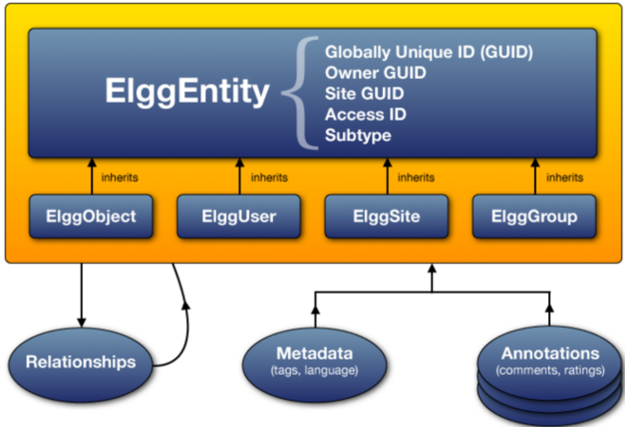
Figura 9: The Elgg data model diagram
